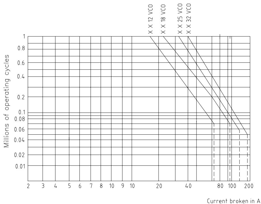
Contactor utilisation category, AC2 ( U_e \leq 440V ) electrical life curve
