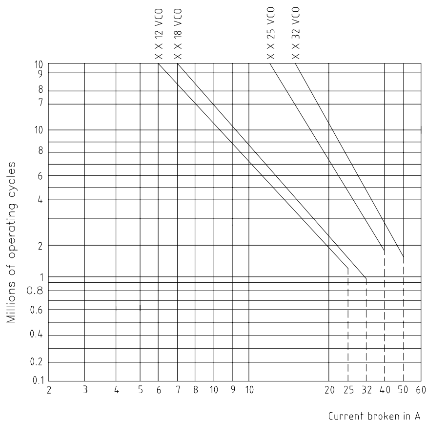
Contactor utilisation category, AC1 ( U_e \leq 440V ) electrical life curve
