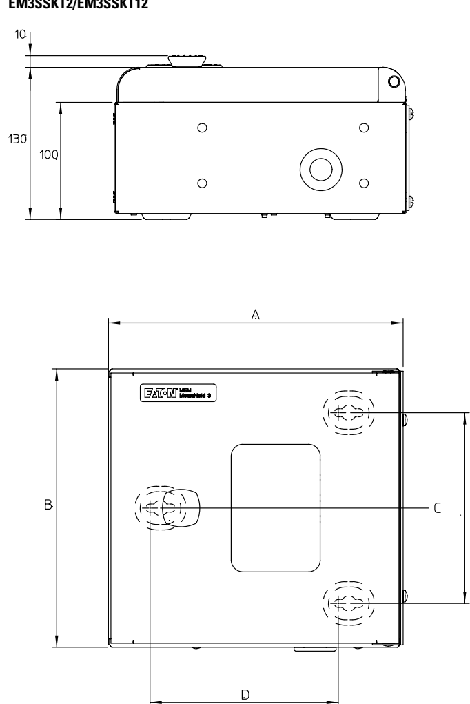
EM3SSK2/EM3SSK12
