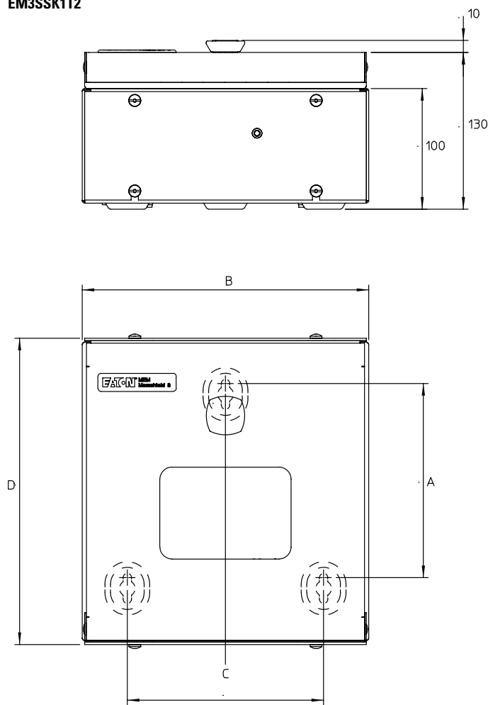
EM3SSK1T2
