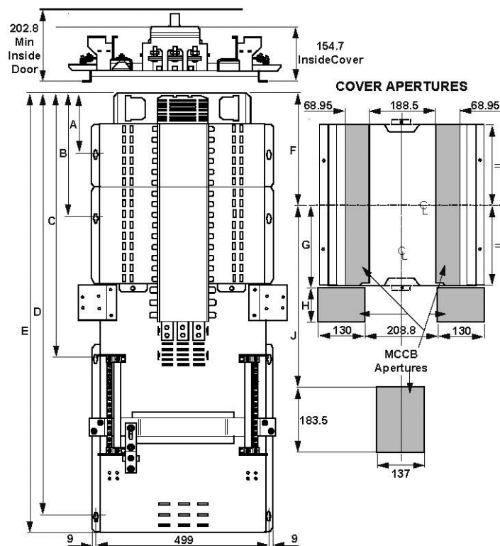
400A pan assembly dimensions EPBPN1640–EPBPN21840
