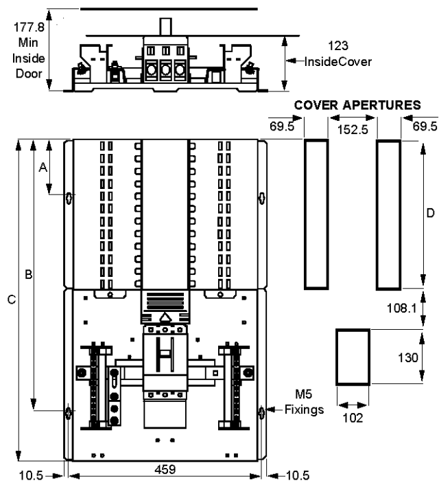
250A pan assembly dimensions EPBPN1425–EPBPN11225
